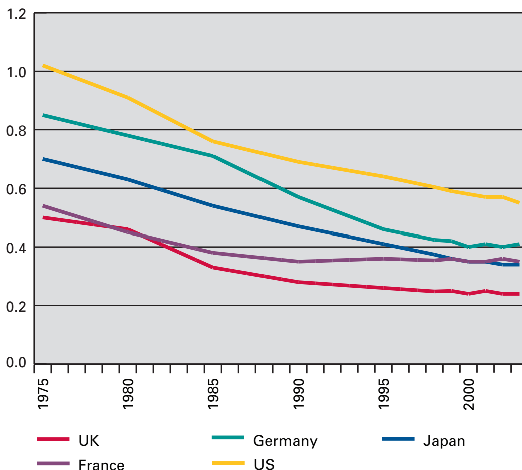
Chart 7: Carbon intensity – energy related CO2 emissions/GDP Mt CO2/GDP (PPP US$ 2000)
