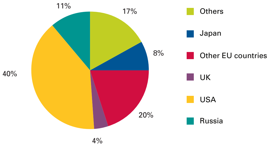
Chart 3: Greenhouse Gas emissions in Annex I countries
